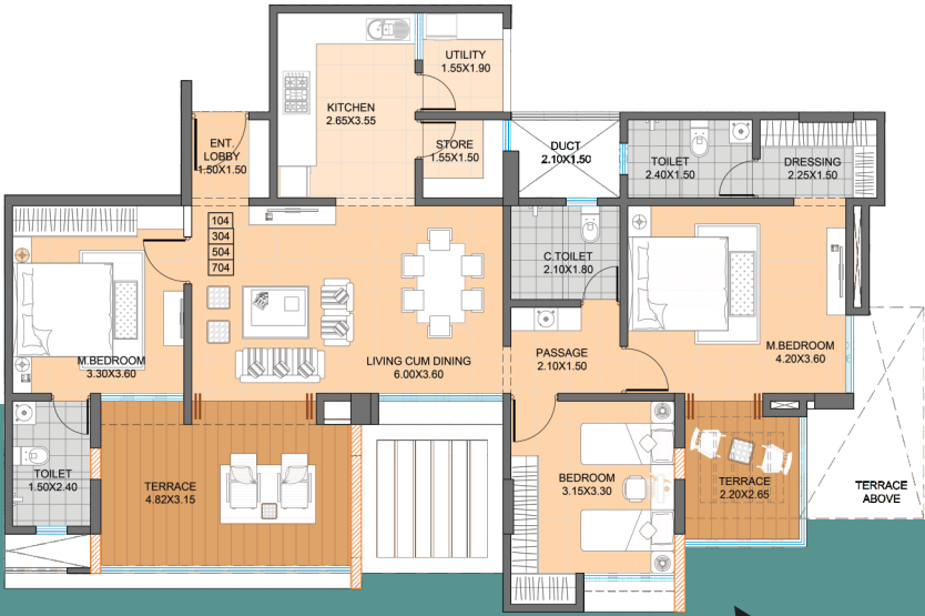
1 st , 3 rd , 5 th , 7 th Floor Plan
