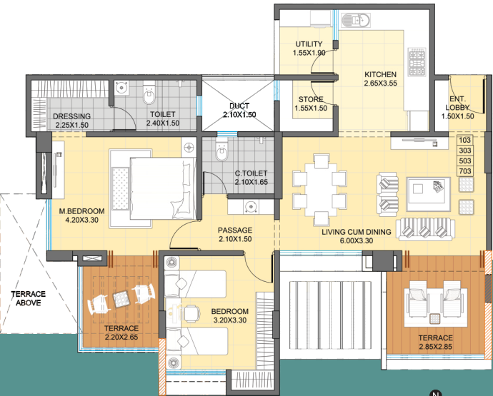
1 st , 3 rd , 5 th , 7 th Floor Plan
